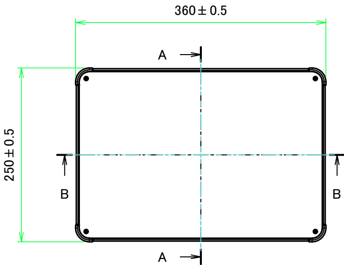
E view
