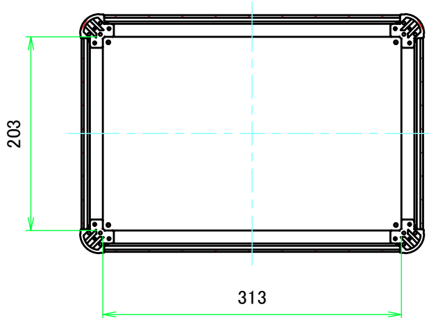
C-C ( 1:5.5 )
